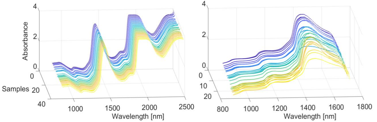
Figure 3 Raw absorbance of spectra of lactate in a) PBS b) human serum c) sheep blood d) invivo human tissue
