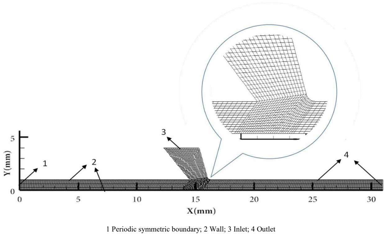
Figure 4. Simulation model and meshes of the jet in polishing zone
