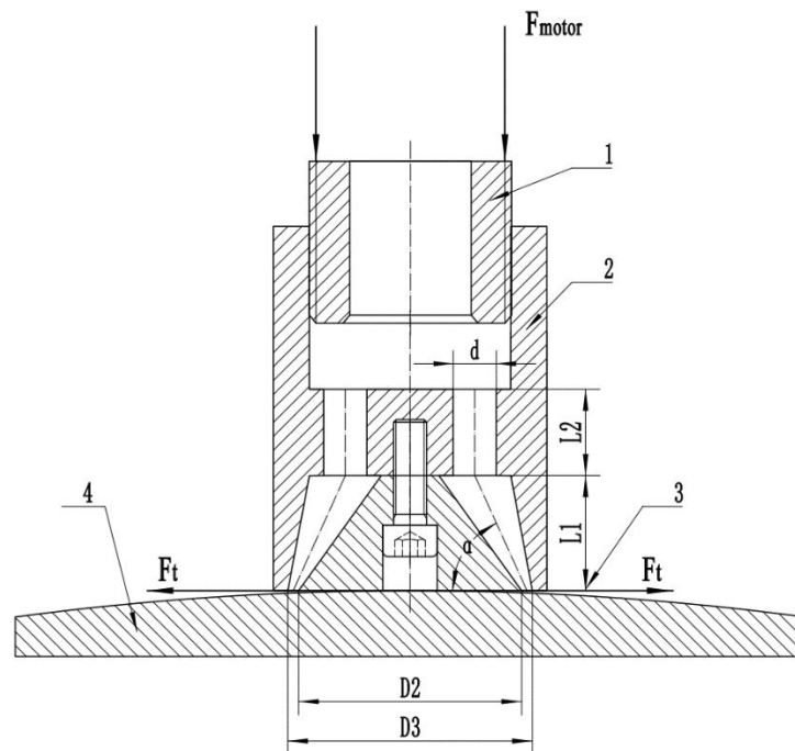
1 Nozzle, 2 shroud, 3 jet, 4 workpiece
