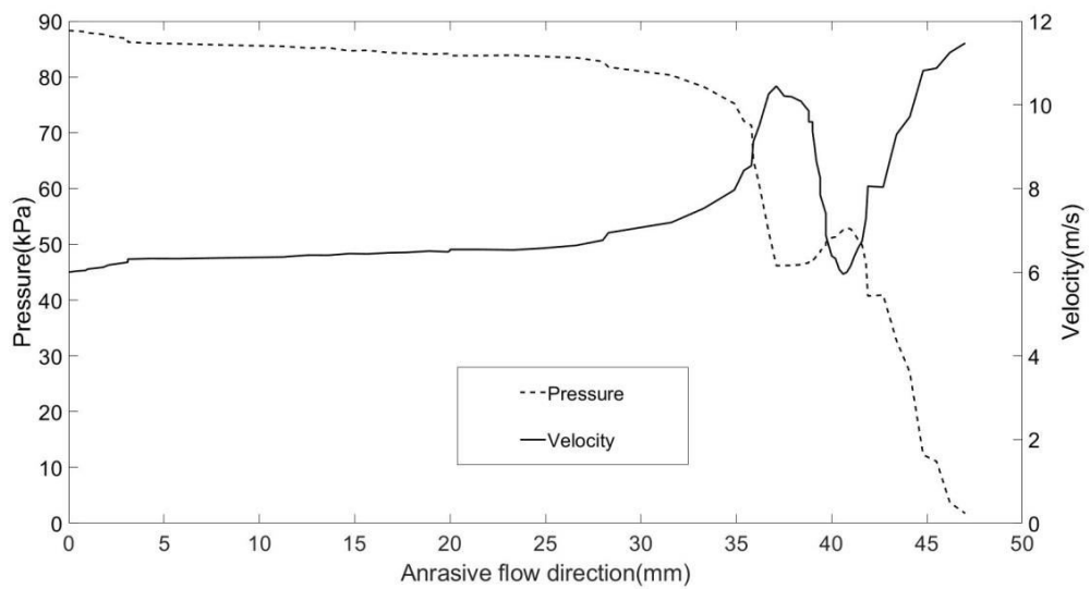
(c) Pressure and speed change along the detection line illustrated in Fig. 2(b)
