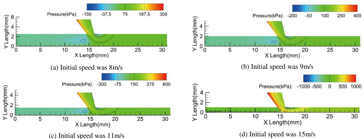
Figure 5. Pressure distribution of abrasive jet in polishing zone
