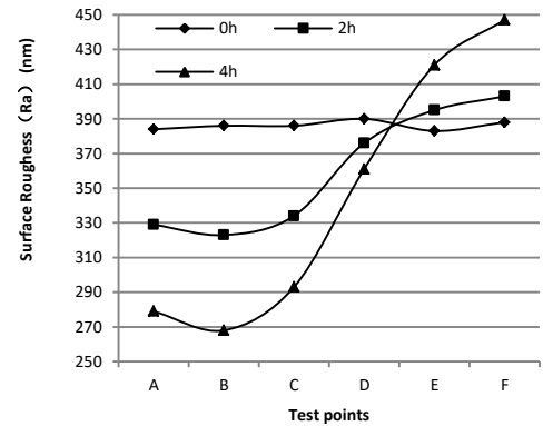
(b) Surface roughness at different test points
