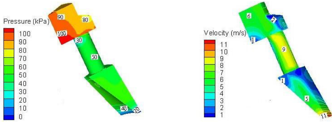
(a) Pressure distribution of internal flow
