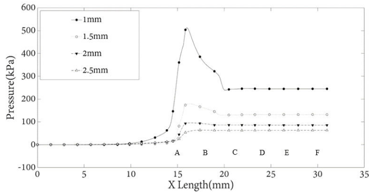
(b) Variation of average pressure along radial direction
