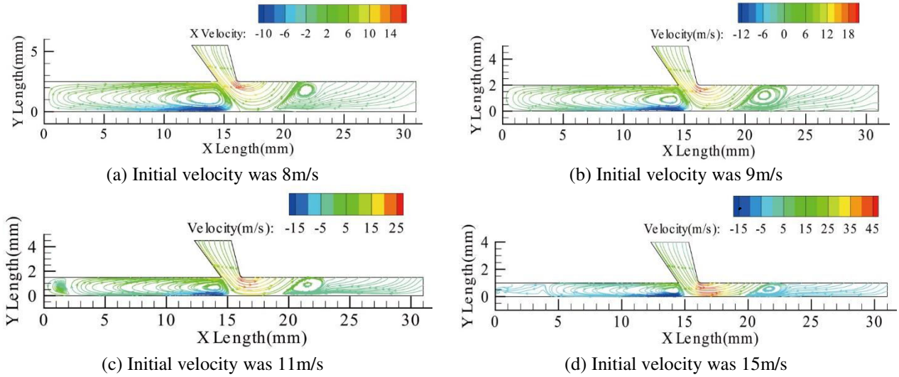
Figure 6. The speed streamline of the abrasive jet flow in polishing zone
