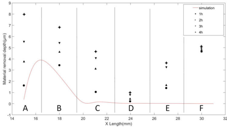
(a) Experimental and simulation results of polishing MMR
