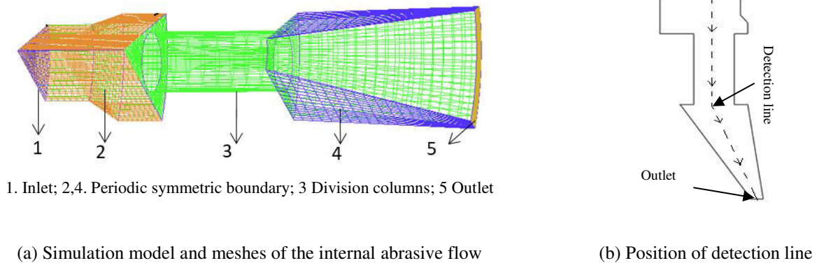
Figure 2. Simulation model and meshes of the internal abrasive flow
