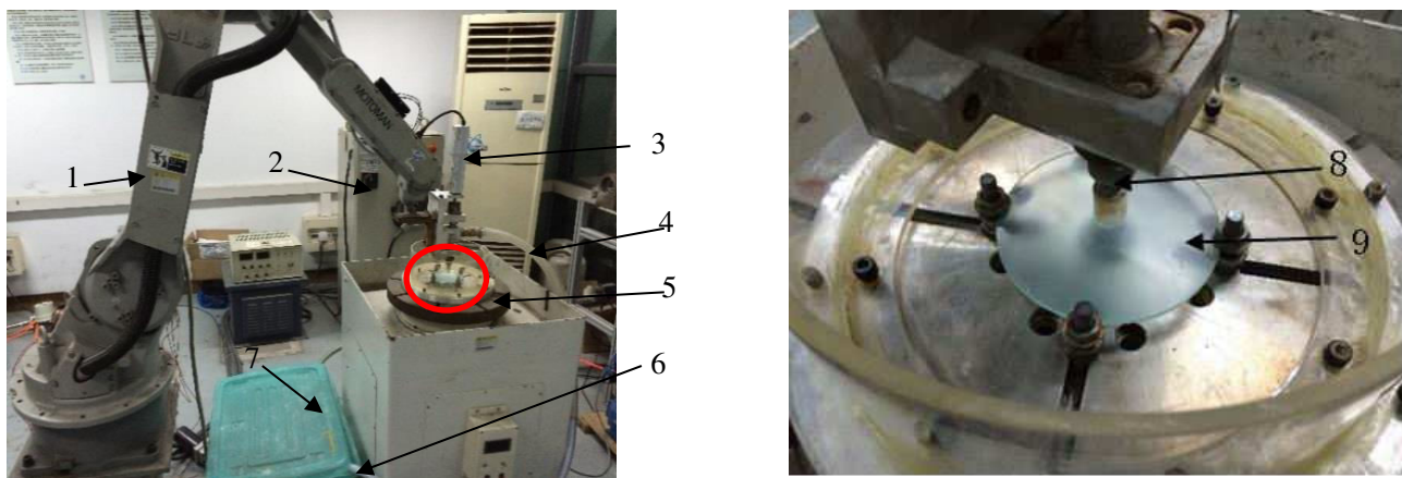
(a) Apparatus setup for AJP process 1. Robot arm, 2. Control cabinet, 3. Step motor, 4. Feeding pipe, 5. Processing platform, 6. Return pipe, 7. Grinding box, 8. CAJP nozzle, 9. Workpiece.
