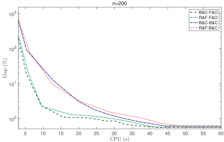
Figure 1: Optimality gap for instances with n = 200
