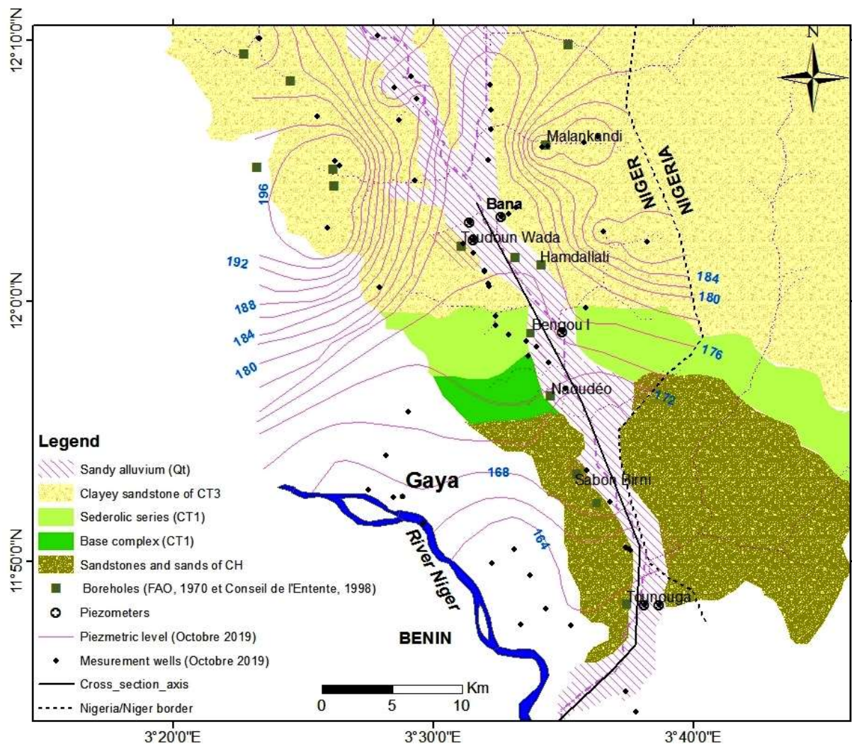
Fig. 2 Surface geology and piezometric contours of the unconfined aquifer in the Dallol Maouri valley and interfluvies of southwestern Niger (BGR/ABN, 2019)
