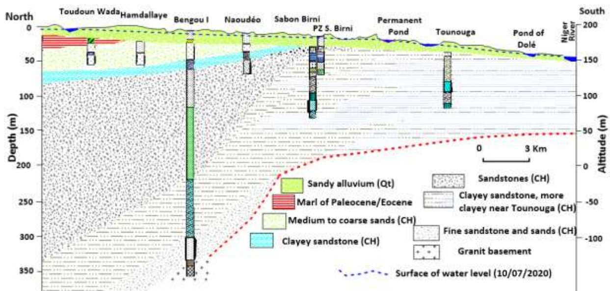
Fig. 3 Geological cross section along the longitudinal axis of the lower Dallol Maouri valley
