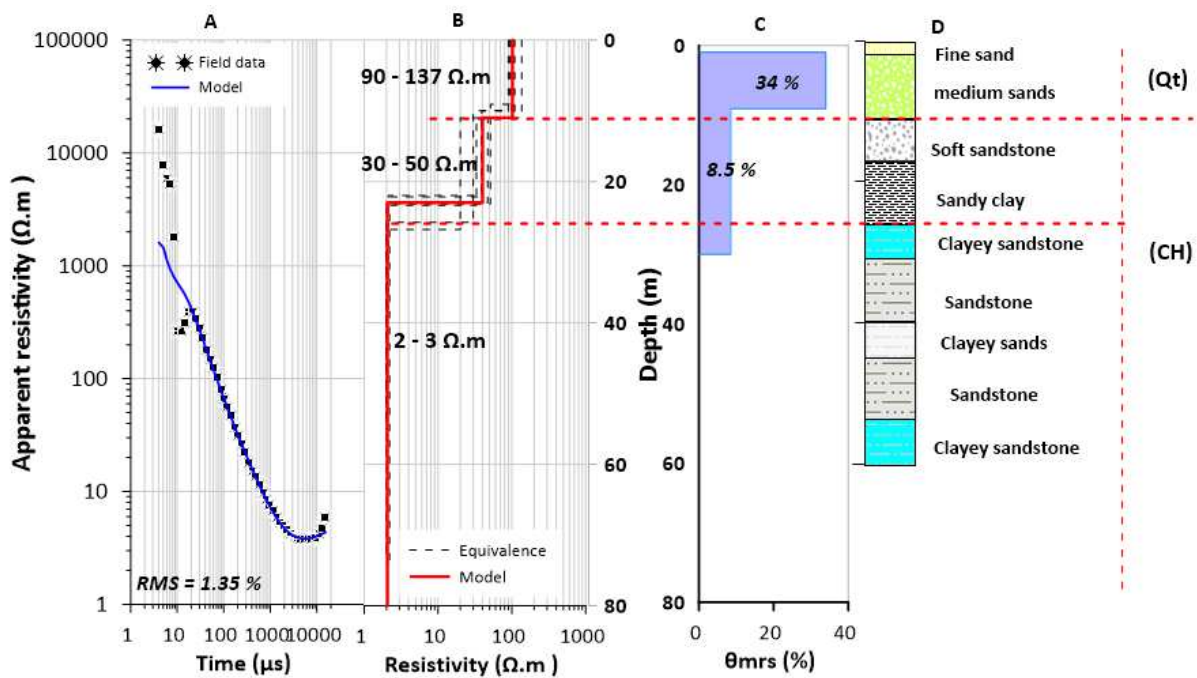
Fig. 4 Interpretation procedure for TDEM and MRS soundings, example of soundings around Bengou I borehole, Bengou cross-section. A : TDEM raw data and the inversion model, B : TDEM results best model and equivalences, MRS results D : geological log of Bengou I borehole
