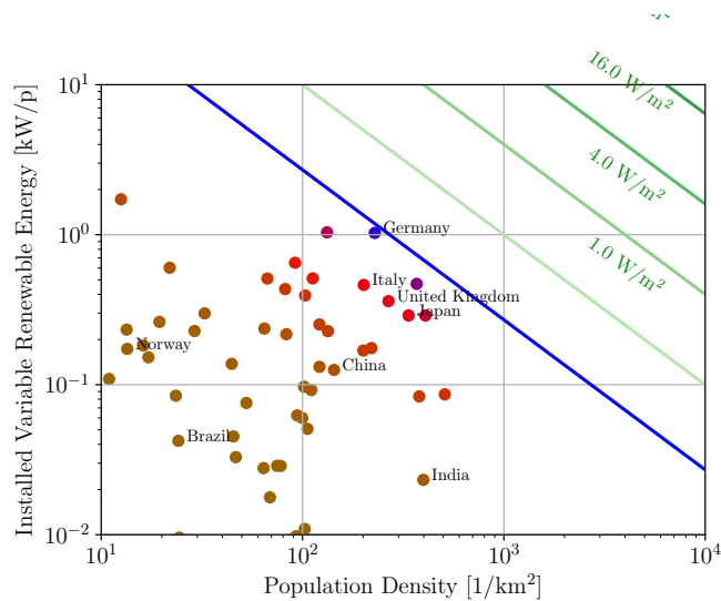
Fig. 4 Installed VRE and population density for 131 countries worldwide (2015 data). 35 The blue trend line represents Germany's (2018) 0.27 \text{ W/m}^2 fit. The green lines represent theoretical solar and wind density calculated theoretical limits of 1.0, 4.0, 16.0 \text{ W/m}^2 .
