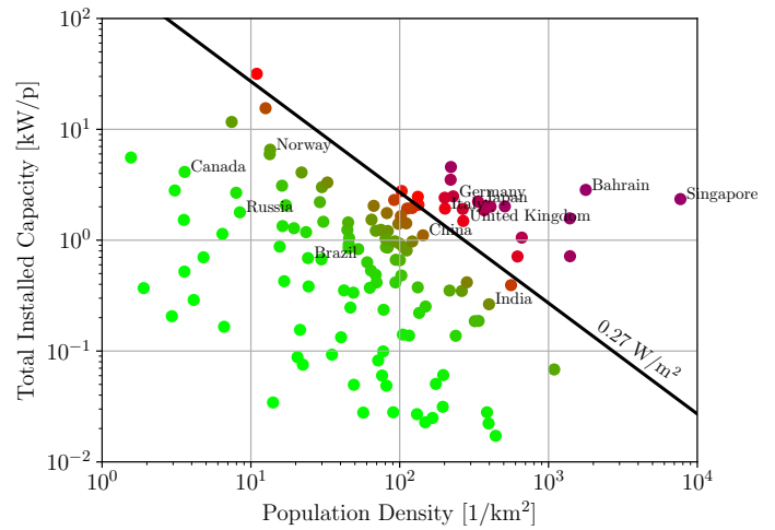
Fig. 5 The installed electricity production capacity and population density for 131 countries worldwide (2015 data). The black trend line represents Germany's 2018 b_c = 0.27 \text{ W/m}^2 value.
