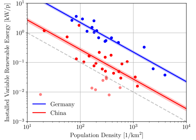
Fig. 2 Germany and China states Installed VRE capacity per capita vs the population density (2015). The blue dots are Germany's states and the blue line shows Germany's 0.23 \pm 0.02 W/m^2 fit. The red dots are China's states and the red line shows China's 0.027 \pm 0.004 W/m^2 gradient. The light gray band stands for the cutoff of 0.001 W/m^2 for states with low power density.
