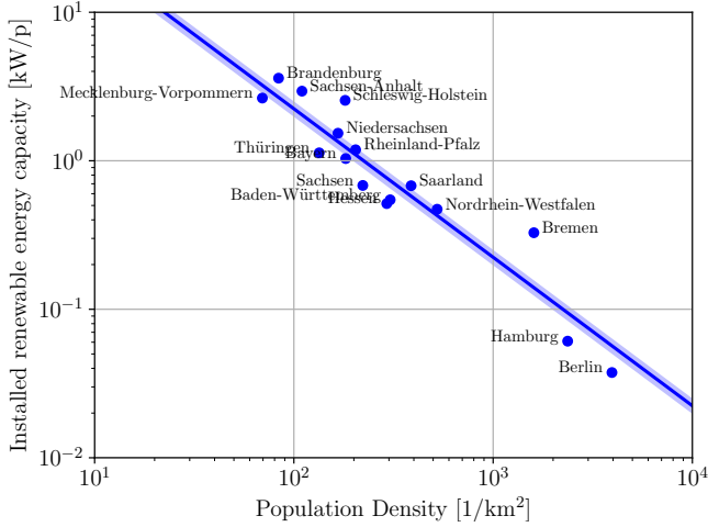
Fig. 1 Installed VRE capacity per capita vs the population density, in the different German states (2015). The blue line results from (3) with the best estimate for b , the light blue band stands for an error of \pm standard deviation in b . Data source: Germany Renewable Energies Agency.
