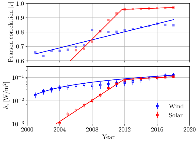
Fig. 3 The correlation between installed VRE capacity per capita and the population density in Germany as a function of time. Top: The absolute value of the Pearson correlation |r| . Bottom: The power density parameter b_c . Blue squares: onshore wind. Red squares: solar. The lines are linear or exponential fits to the data.
