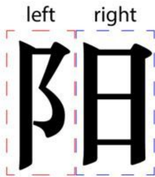
Left-right construction
