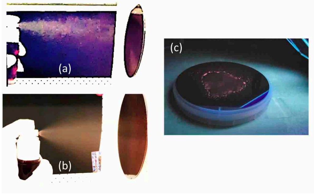
Figure 2. (a) and (b) Optimizing the spray coating pattern on a Si wafer. The spray cloud under exposure of UV radiation with a wavelength of 365 nm (c) An example of a Si wafer under UV irradiation after spraying the Si NPs.
