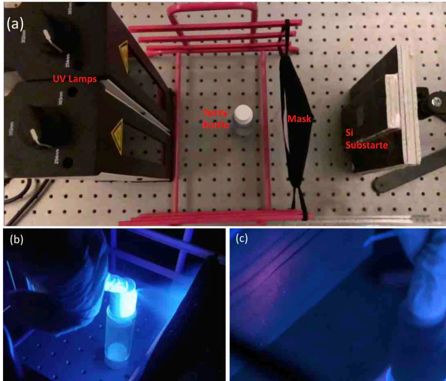
Figure 3. (a) Top view of the setup used to spray the masks (b) Spray pattern from the spray bottle (c) Spraying the mask under the UV lamp
