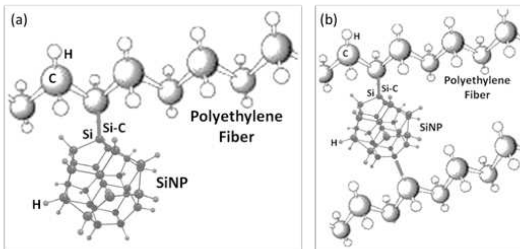
Figure 10. (a) The Si-C bond form between the bare silicon and the carbon atoms in PE. (b) The Si NP interacting with multiple PE chain while the nanoparticle acts a secondary cross linker.
