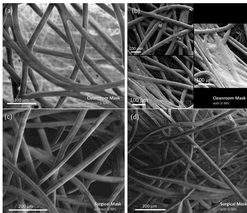
Figure 4 Scanning electron microscope image of the (a-b) cleanroom and (c-d) surgical mask with and without Si nano particles.
