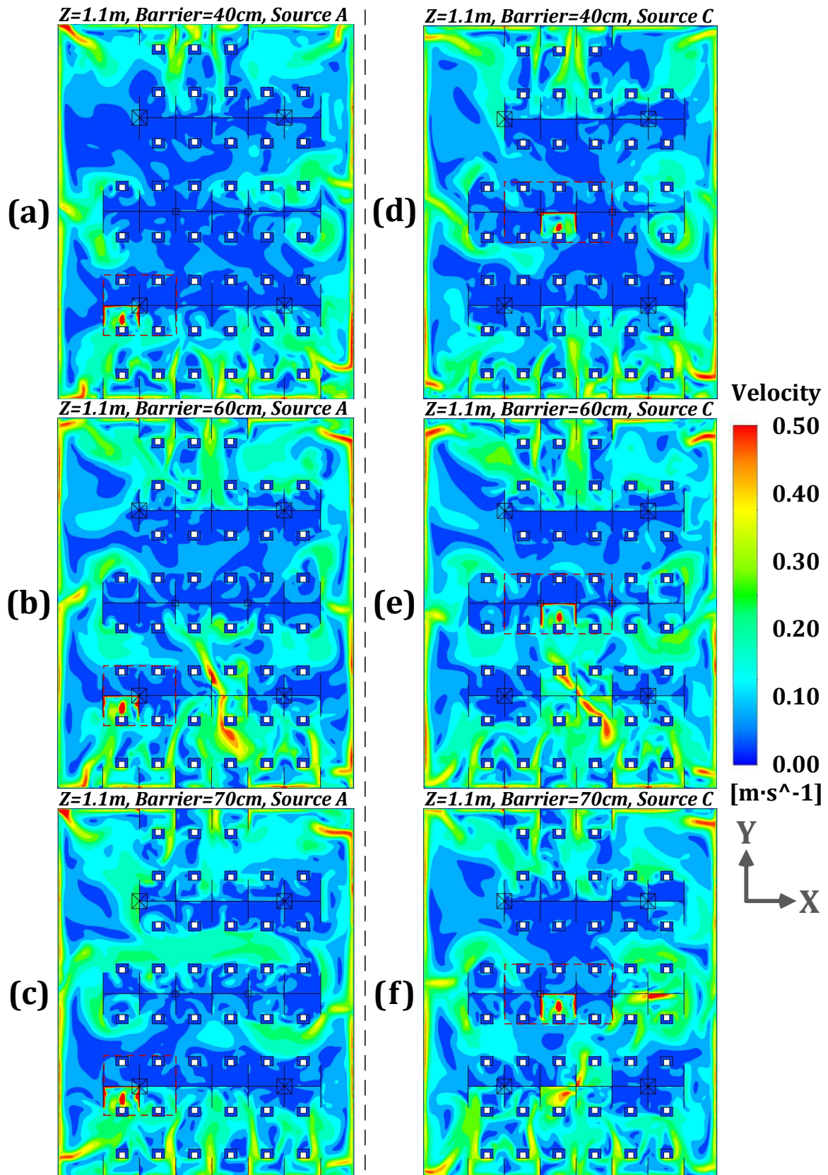
Fig. 11. Airflow distributions at the plane of z=1.1m with the barrier heights of 40, 60 and 70cm under modified ventilation mode and pollution sources of A and C [(a): height of 40cm and source of A; (b): height of 60cm and source of A; (c): height of 70cm and source of A; (d): height of 40cm and source of C; (e): height of 60cm and source of C; (f): height of 70cm and source of C].
