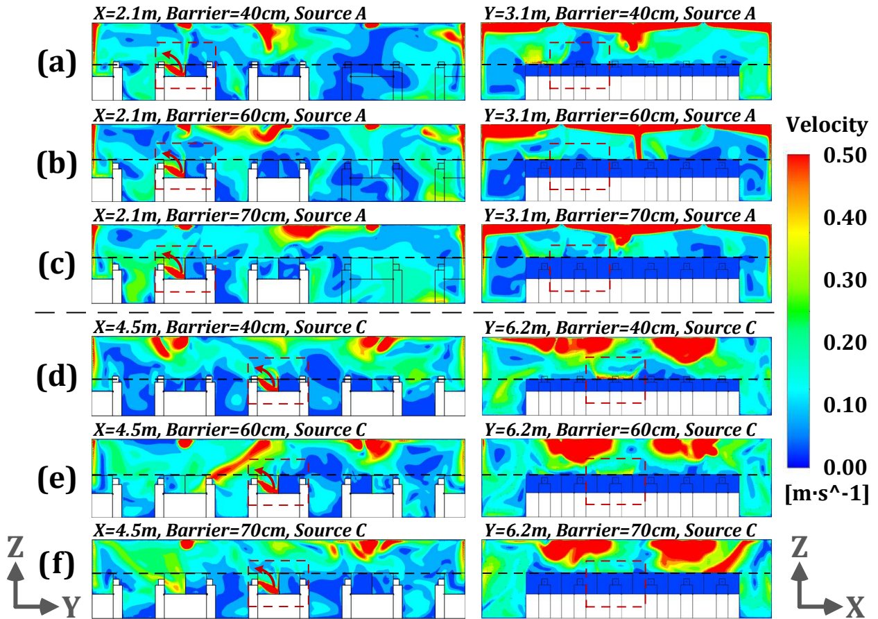
Fig. 10. Airflow distributions for different profiles with the barrier heights of 40, 60 and 70cm and pollution source located A and C [(a): planes of x=2.1\text{m} and y=3.1\text{m} with barrier height of 40cm and source at point A; (b): planes of x=2.1\text{m} and y=3.1\text{m} with barrier height of 60cm and source at point A; (c): planes of x=2.1\text{m} and y=3.1\text{m} with barrier height of 70cm and source at point A; (d): planes of x=4.5\text{m} and y=6.2\text{m} with barrier height of 40cm and source at point C; (e): planes of x=4.5\text{m} and y=6.2\text{m} with barrier height of 60cm and source at point C; (f): planes of x=4.5\text{m} and y=6.2\text{m} with barrier height of 70cm and source at point C].
