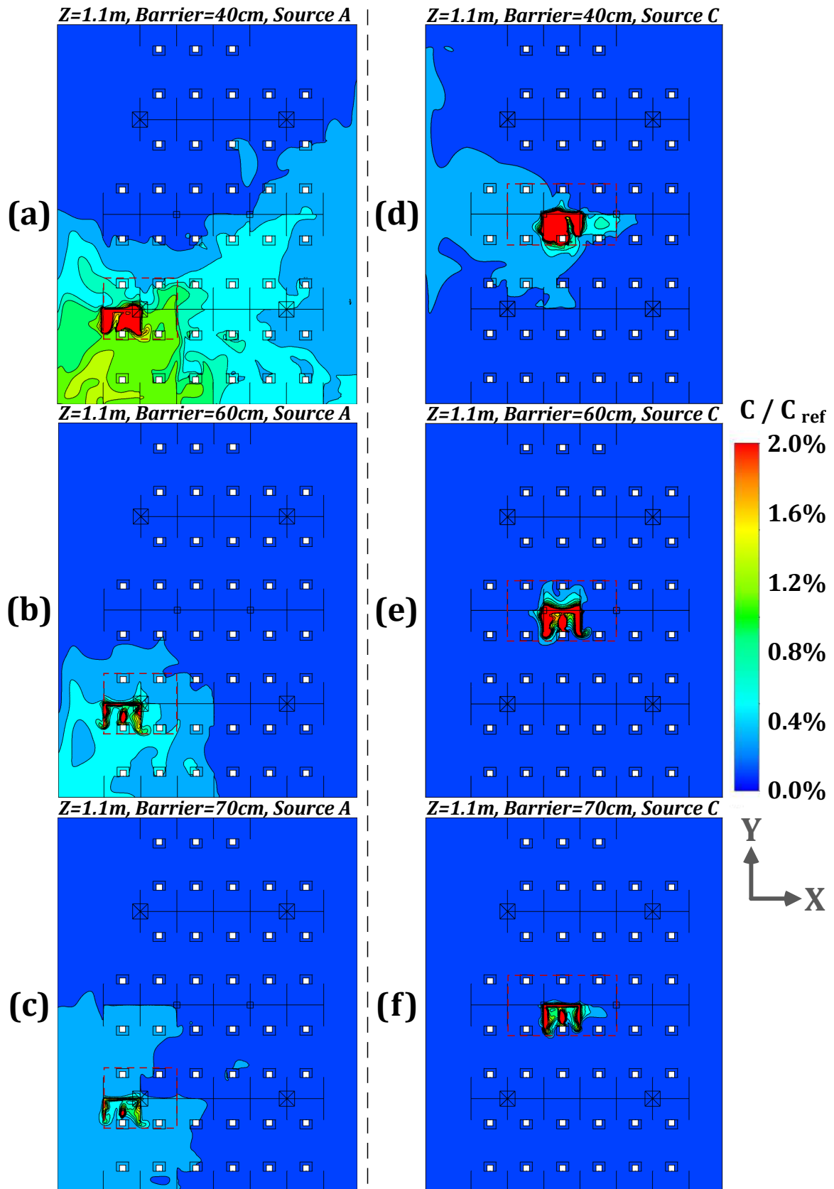
Fig. 15. Pollutant concentrations ( C/C_{ref} ) at the plane of z=1.1m under modified ventilation mode with the barrier heights of 40, 60 and 70cm and pollutant sources at point A and C [(a): height of 40cm and source at A; (b): height of 60cm and source at A; (c): height of 70cm and source at A; (d): height of 40cm and source at C; (e): height of 60cm and source at C; (f): height of 70cm and source at C].
