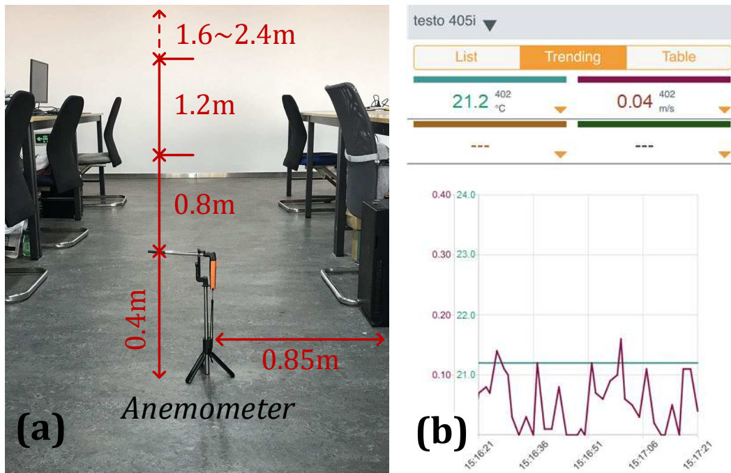
Fig. 5 Schematic diagram of on-site monitoring setup in the office (a): layout of thermal anemometer; (b): monitoring interface for smartphone
