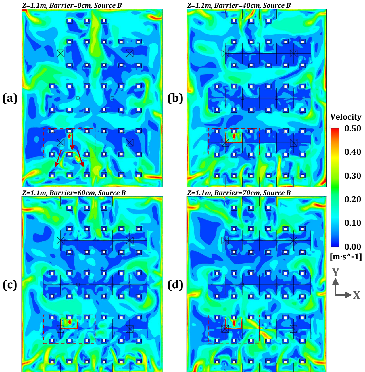
Fig. 9. Airflow distributions at the plane of z=1.1\text{m} with the barrier heights of 0, 40, 60 and 70cm under modified ventilation system and pollution source B [(a): height of 0cm; (b): height of 40cm; (c): height of 60cm; (d): height of 70cm].
