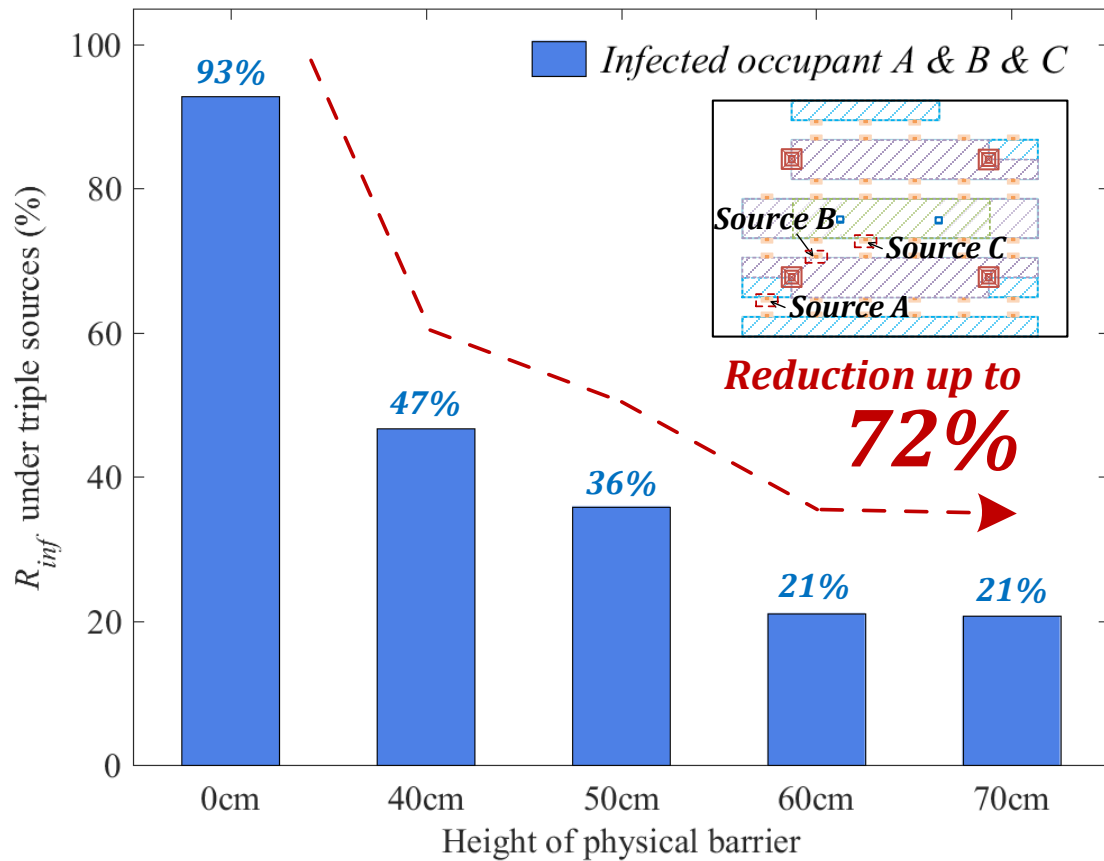
Fig. 17. Infection risk (exposure time is 1 hour) for multiple pollutant sources (A, B and C) with modified ventilation mode and barrier heights of 0, 40, 50, 60 and 70cm.
