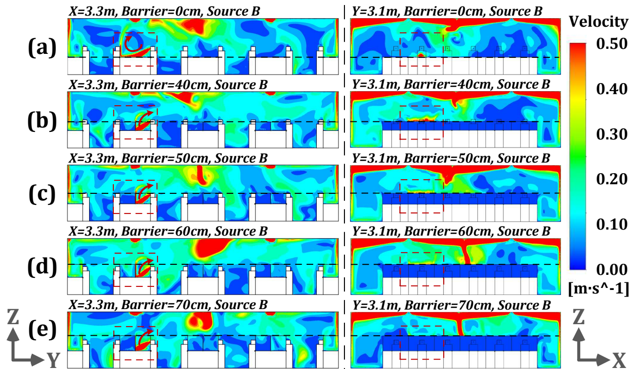
Fig. 8. Airflow distributions at the planes of x=3.3\text{m} and y=3.1\text{m} with the barrier heights of 0, 40, 50, 60 and 70cm under modified ventilation mode and pollution source of B [(a): height of 0cm; (b): height of 40cm; (c): height of 50cm; (d): height of 60cm; (e): height of 70cm].
