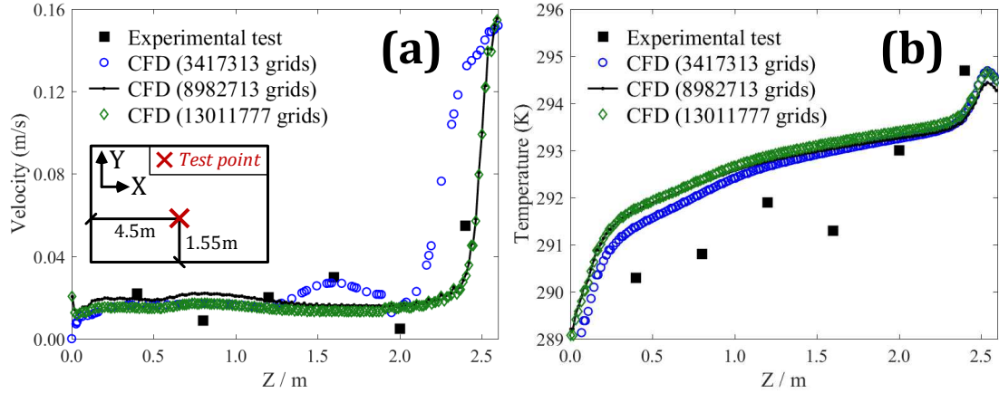
Fig. 6. Validations between experimental tests and numerical simulations as well as the grid independence analysis (a): airflow velocity; (b): indoor temperature.
