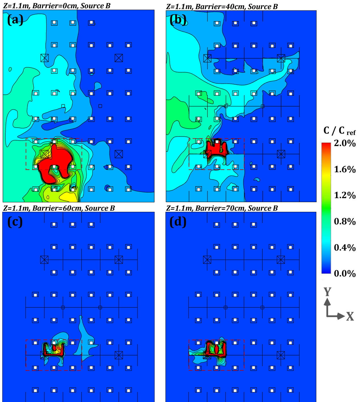
Fig. 13. Pollutant concentrations ( C/C_{ref} ) for the plane of z=1.1m under modified ventilation mode with the barrier heights of 0, 40, 60 and 70cm and pollutant source at point B [(a): height of 0cm; (b): height of 40cm; (c): height of 60cm; (d): height of 70cm].
