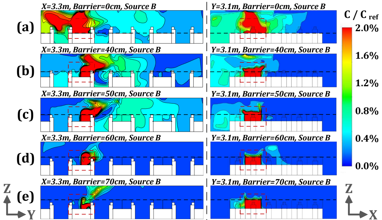
Fig. 12. Pollutant concentrations ( C/C_{ref} ) for the planes of x=3.3m and y=3.1m under modified ventilation mode with the barrier heights of 0, 40, 50, 60 and 70cm and pollutant source at point B [(a): height of 0cm; (b): height of 40cm; (c): height of 50cm; (d): height of 60cm; (d): height of 70cm].
