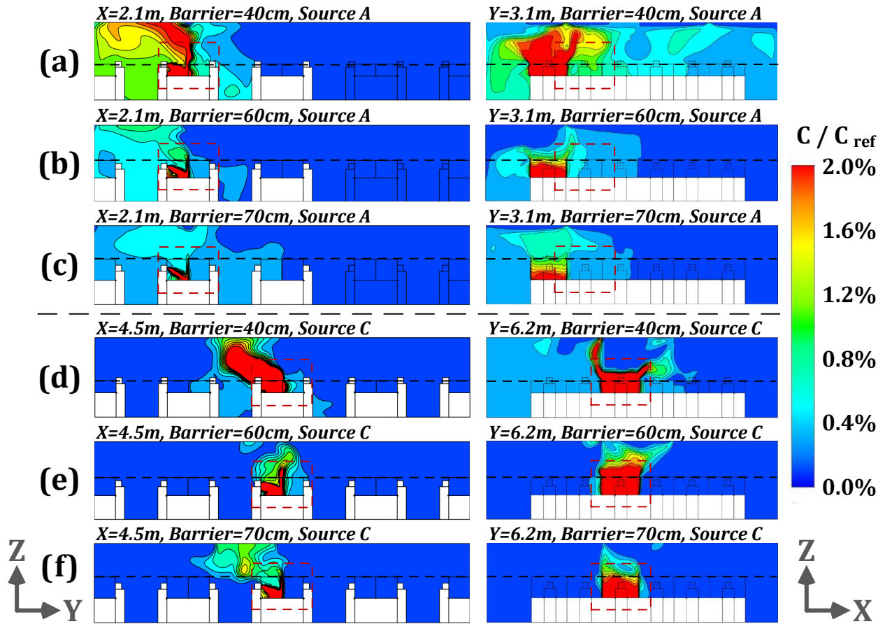
Fig. 14. Pollutant concentrations ( C/C_{ref} ) for different profiles under modified ventilation mode with the barrier heights of 40, 60 and 70cm and pollutant sources located at A and C [(a): planes of x=2.1m and y=3.1m with barrier height of 40cm and source at point A; (b): planes of x=2.1m and y=3.1m with barrier height of 60cm and source at point A; (c): planes of x=2.1m and y=3.1m with barrier height of 70cm and source at point A; (d): planes of x=4.5m and y=6.2m with barrier height of 40cm and source at point C; (e): planes of x=4.5m and y=6.2m with barrier height of 60cm and source at point C; (f): planes of x=4.5m and y=6.2m with barrier height of 70cm and source at point C].
