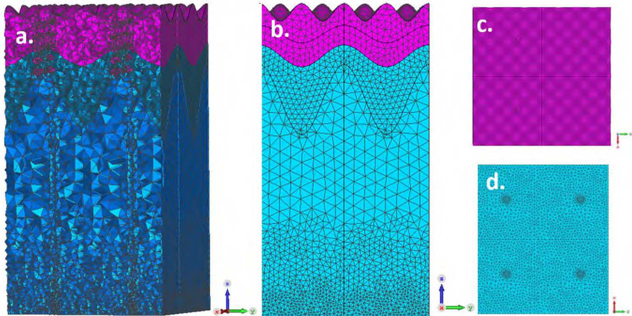
Figure 5. Mesh view of the human skin model. a) a 3D view of the zy-plane, b) a 2D view of the zy-plan. The adaptive mesh is clearly shown, as different areas of the model have different division of tetrahedral mesh cells, c) top view. A more fine division to mesh cells is taking place due to the curved sinusoidal nature of this surface. D) Bottom view. Here, as well, a finer mesh division is taking place to overcome the sharp edges of this surface. This figure was generated using CST STUDIO SUITE v2021 32 , https://www.3ds.com/products-services/simulia/products/cst-studio-suite/ .
