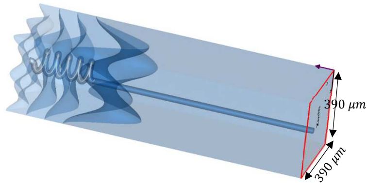
Figure 6. Electromagnetic excitation signal applied to the Z_{min} port, using 18 modes of Floquet. This figure was generated using CST STUDIO SUITE v2021 32 , https://www.3ds.com/products-services/simulia/products/cst-studio-suite/ .
