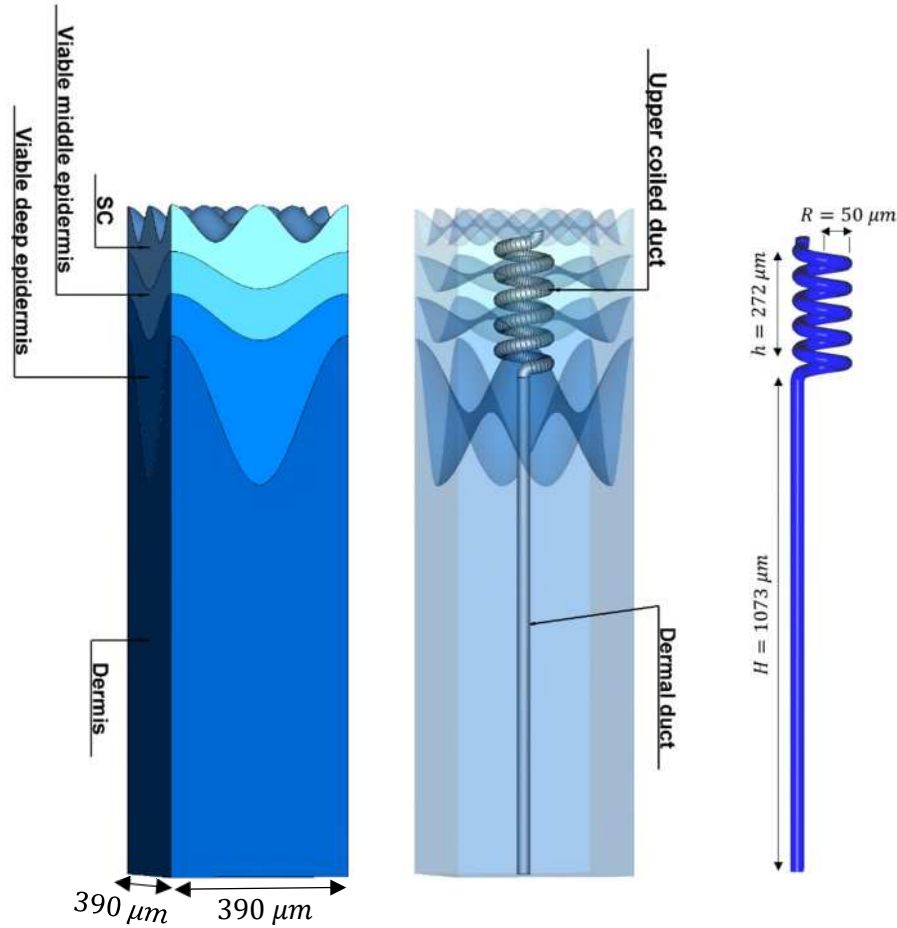
Figure 4. Electromagnetic thick human skin model designed and simulated using CST STUDIO SUITE, MICROWAVE STUDIO 32 . On the left – the whole model from an external view. On the middle – and interior view. As can be seen the coiled duct is fully embedded in the epidermis layer and the dermal duct is fully embedded in the dermis layer. On the right – the sizes of the duct which was used in the simulations. These values were based on the dimension of the layers and the sweat duct obtained in ref 17. The unit cell dimensions are 390 \mu\text{m} \times 390 \mu\text{m} . This figure was generated using CST STUDIO SUITE v2021, https://www.3ds.com/products-services/simulia/products/cst-studio-suite/ .
